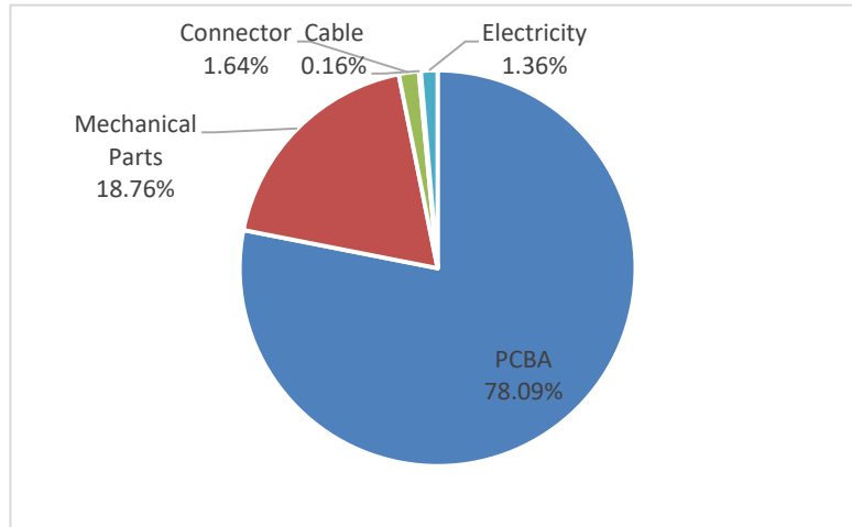
Figure 4 Product Carbon footprint analysis by manufacturing process
